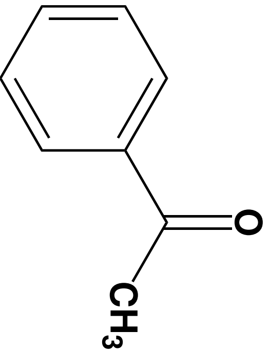
Acetophenone
