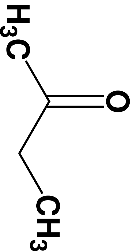
2-butanone
