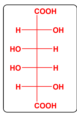
Galactaric Acid meso; optically inactive
