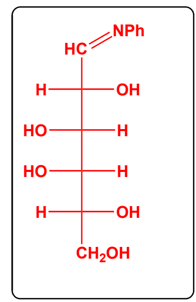
Shiff Base of Galactose
