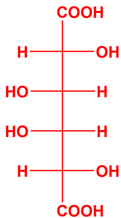
Galactaric Acid meso; optically inactive
